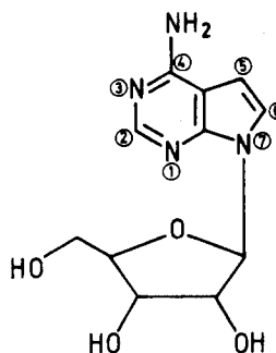
Tubercidin
